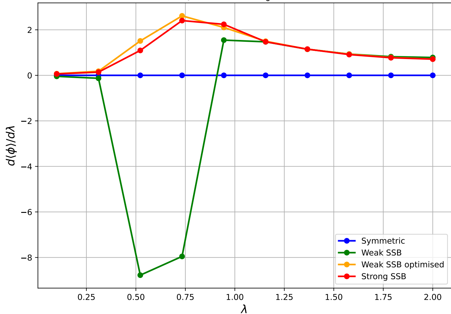
d\langle\phi\rangle/d\lambda vs \lambda , m_0^2 = -2.0
